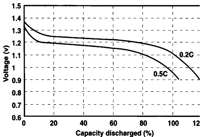
Discharge curves of single cell EH-60B16 at -8°C at various discharge rates at room temperature
