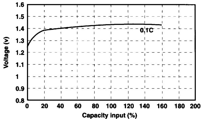
Charging curve of single cell EH-60B16 -80mAh at 0.1C charging rate
